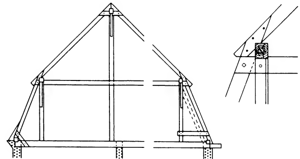
6 Mansard roof
